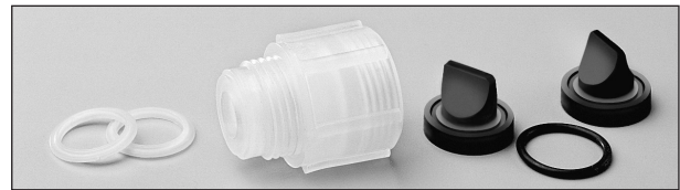
1/2", 3/4", 1", 1 1/2" and 2" Duckbill Valve Kits (Valve extension required only on suction port.)
