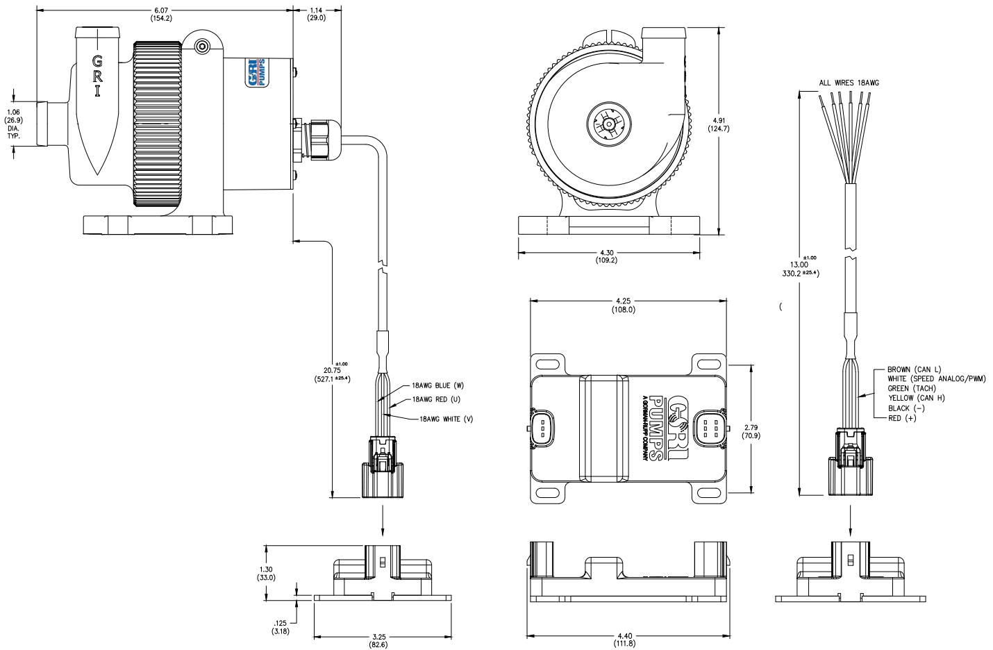
INTG6 Series Typical Dimensional Drawing. OEM options are available. Please contact GRI to discuss.
